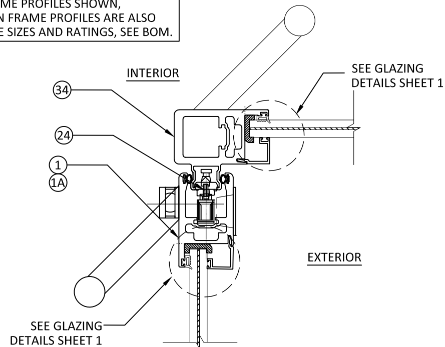
C6 HORIZONTAL SECTION INSIDE CORNER DETAIL
