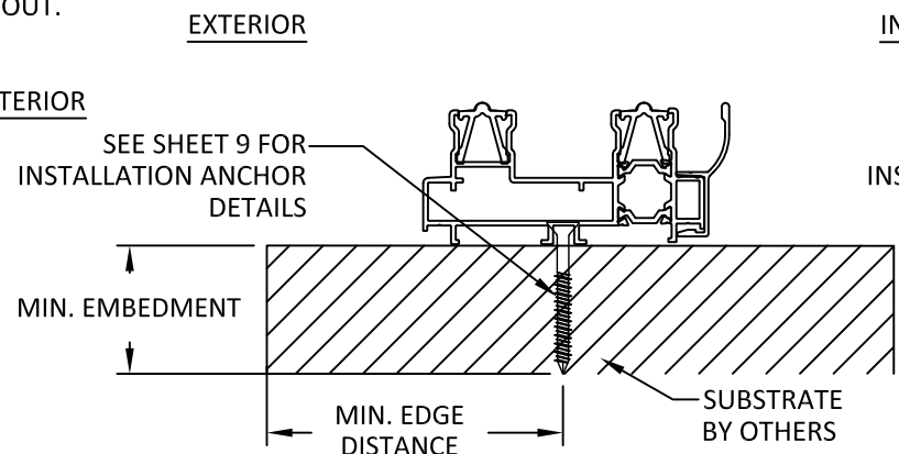
F 8 ANCHOR DETAIL THROUGH FRAME INSTALLATION (SILL) 2 TRACKS
