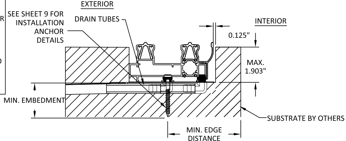
B 8 ANCHOR DETAIL THROUGH FRAME INSTALLATION (HEAD) 2 TRACKS
