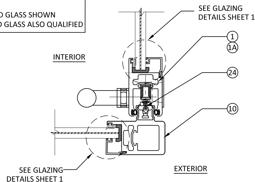
B HORIZONTAL SECTION 6 OUTSIDE CORNER DETAIL
