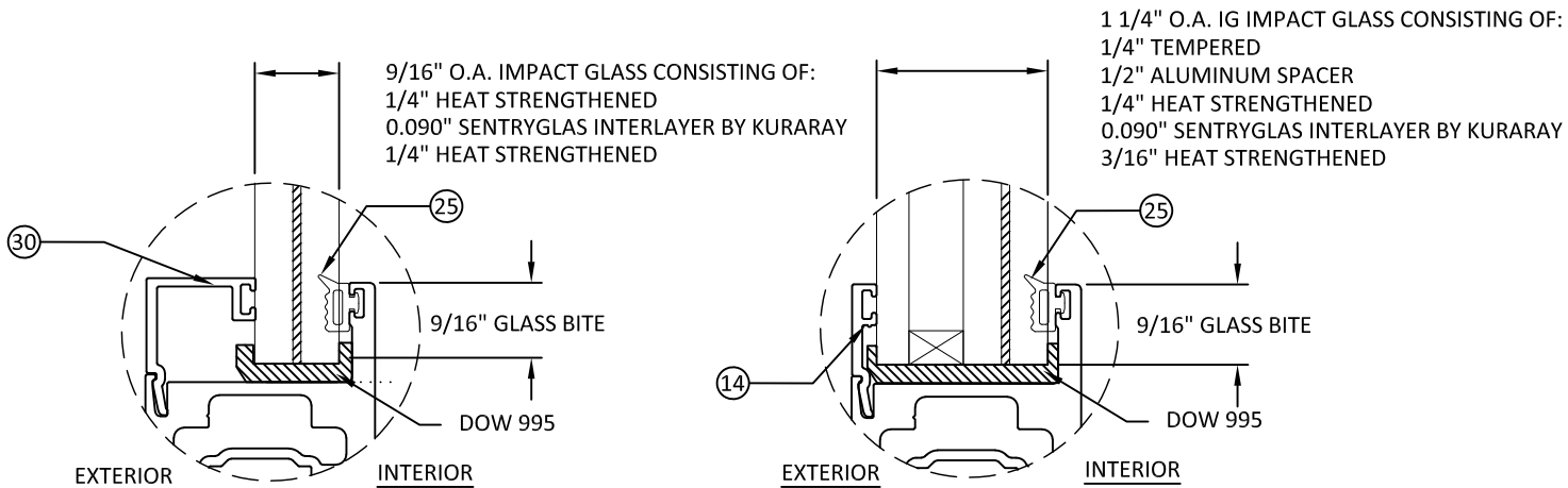
GLAZING DETAIL 1
