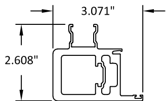
34 INSIDE CORNER ASTRAGAL STILE/SASH 6063-T5
